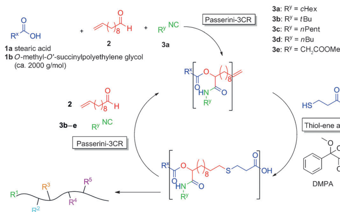
Scheme 1. Synthesis of a sequence-defined tetramer (starting from 1a ) or a sequence-defined block copolymer (starting from 1b ) by iterative application of the P-3CR and the thiol–ene addition reaction.
