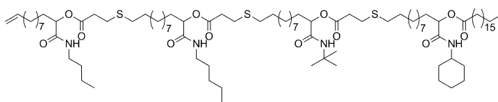
Figure 1. Structure of the obtained sequence-defined tetramer having four different side chains.
