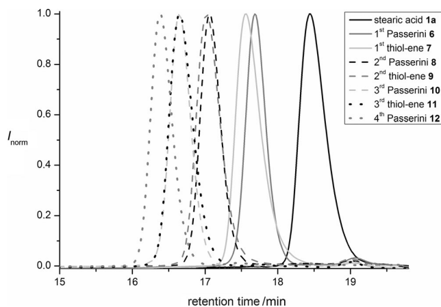
Figure 2. GPC traces obtained after P-3CR and thiol–ene addition reactions in the synthesis of the sequence-defined tetramer.
