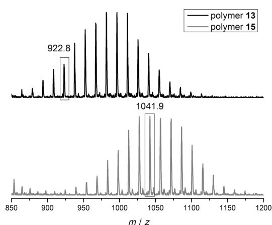
Figure 4. ESI mass spectra of 13 and 15 , showing a shift of the molecular weight distribution towards higher molecular weights. The peaks shown in the spectra correspond to chains carrying three sodium ions and the selected peaks correspond to polymer chains having 51 PEG monomer units.
