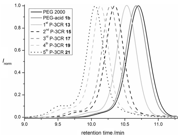
Figure 3. GPC traces of the PEG copolymer after each P-3CR.
